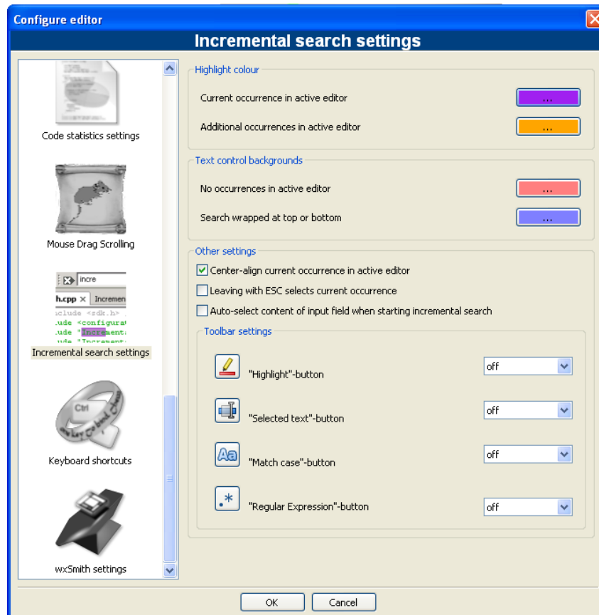
Figure 2.4: Settings for Incremental Search
